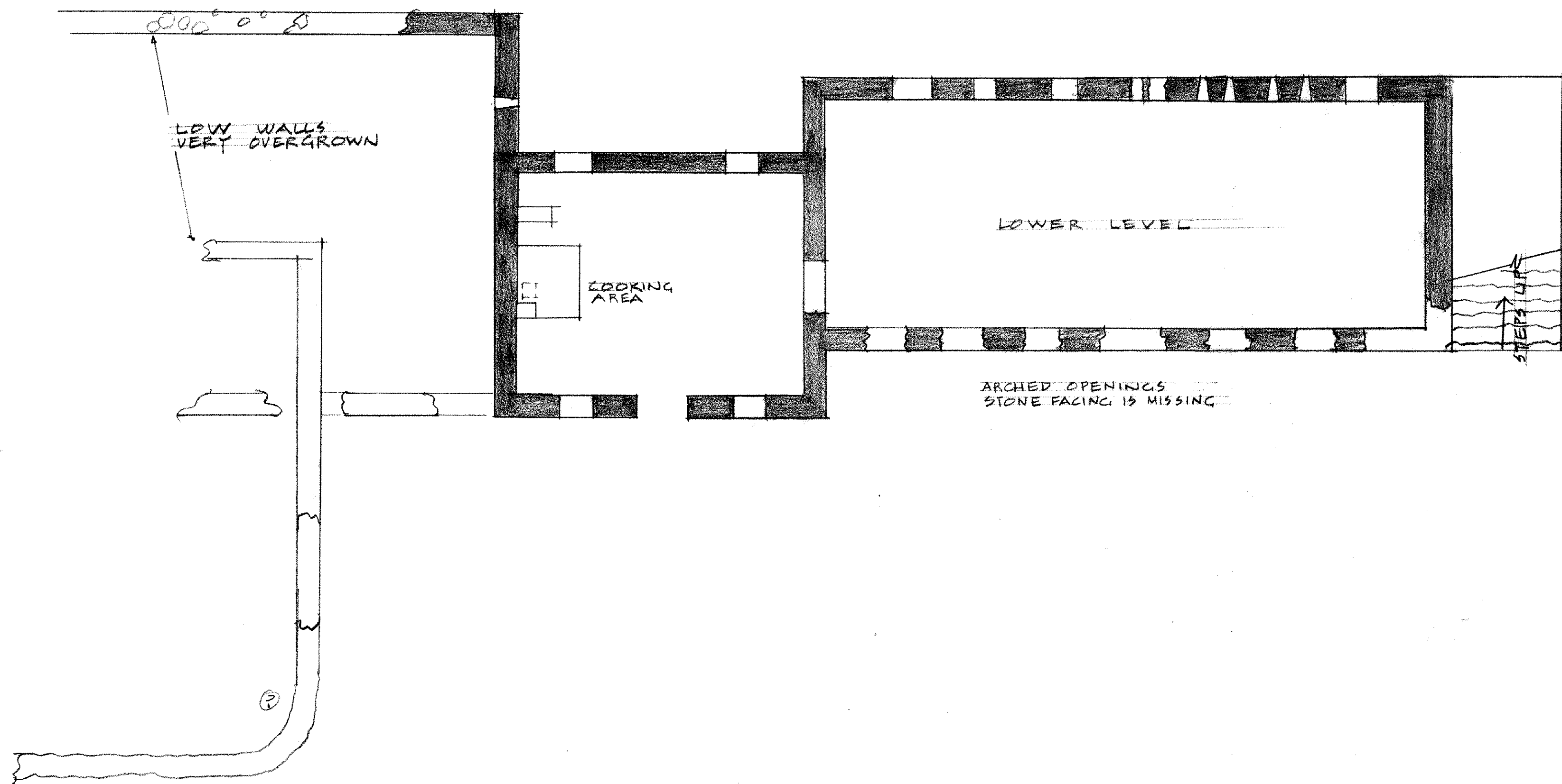
BUILDING COMPLEX #1 1/8" = 1'
